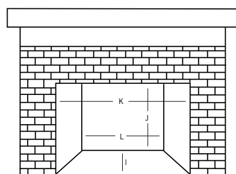
*Illustrations apply to Montlake™
